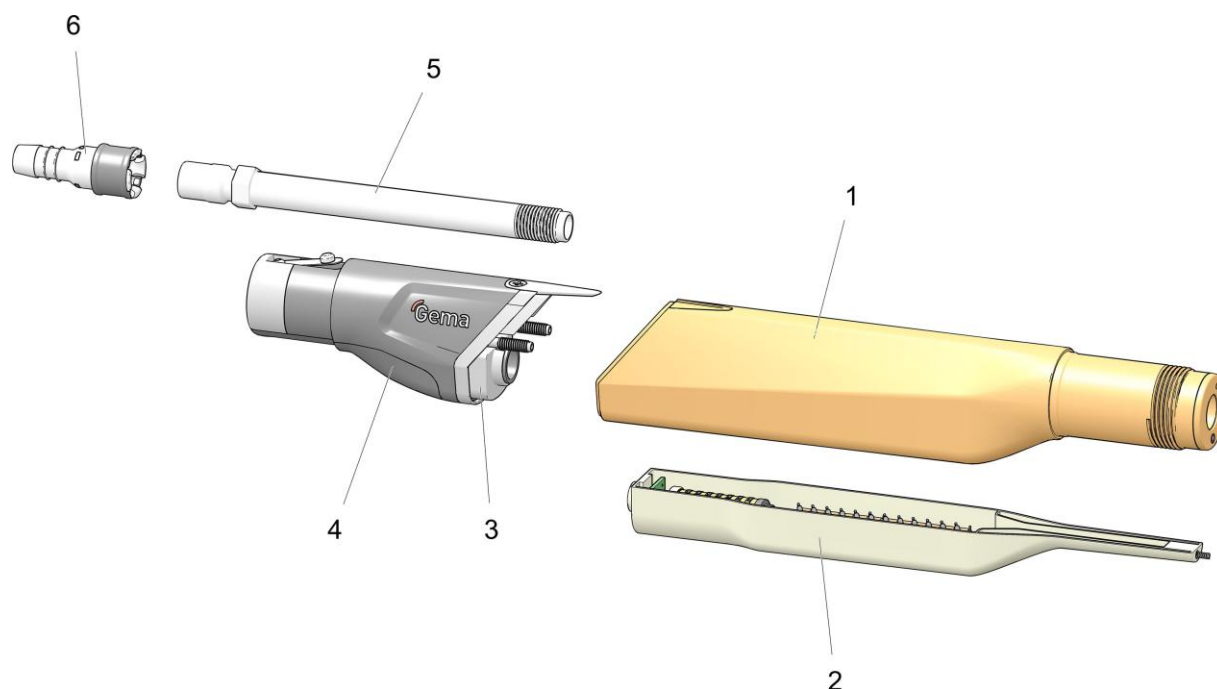
Fig. 11: OptiGun GA04 – gun body
