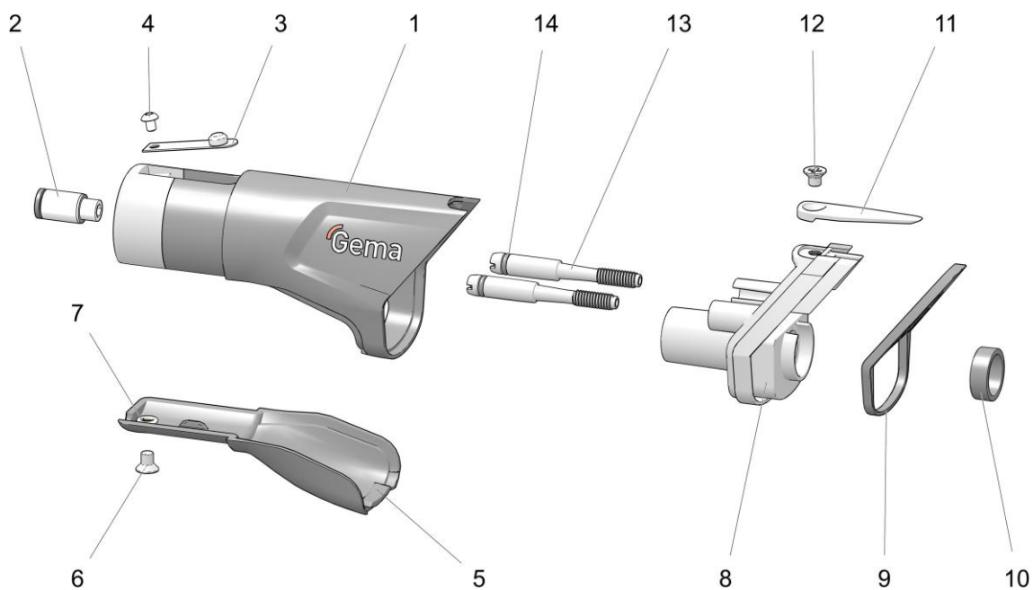
Fig. 12: Gun rear piece
