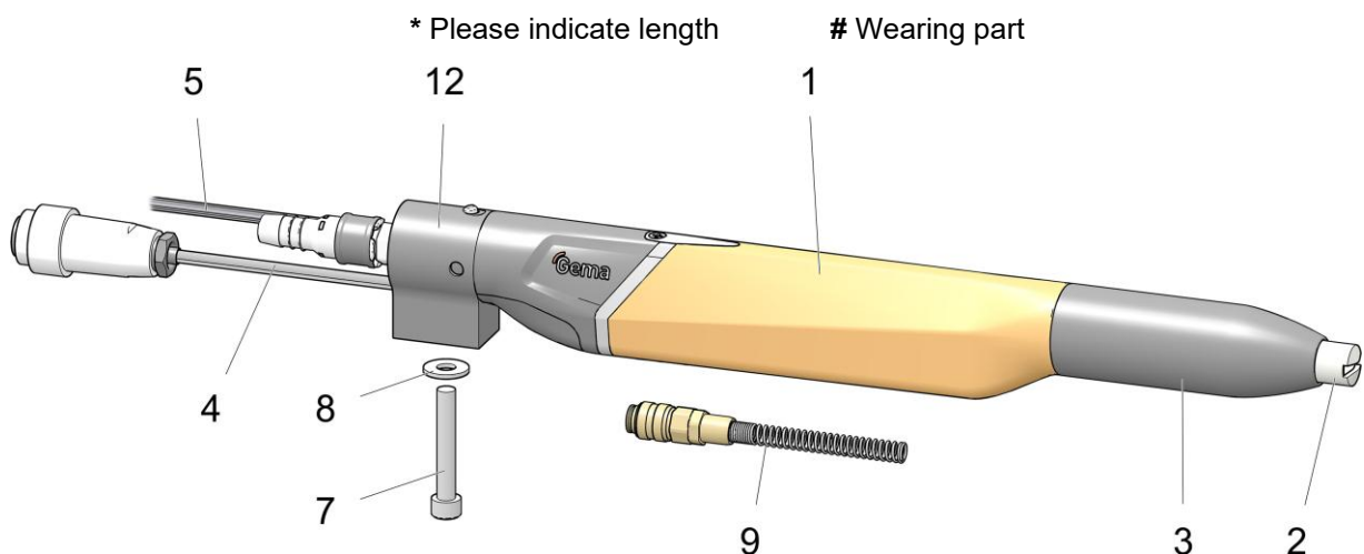
Fig. 10: OptiGun GA04 – complete
