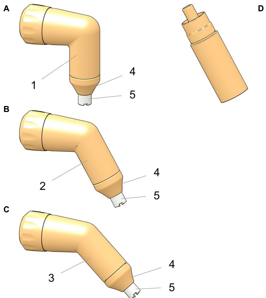
Fig. 18: Angled nozzles
