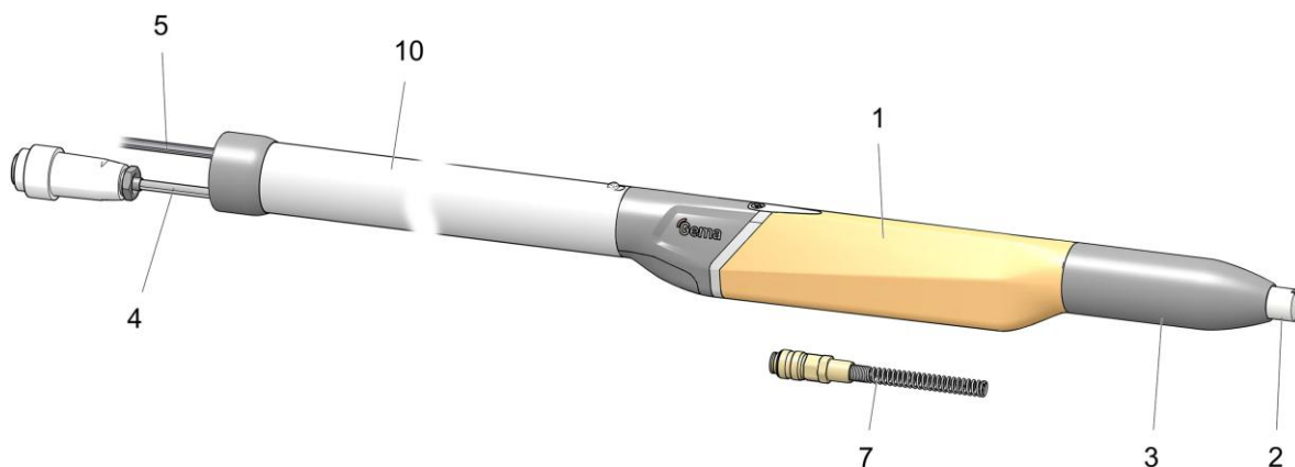
Fig. 13: OptiGun GA04-X – complete
