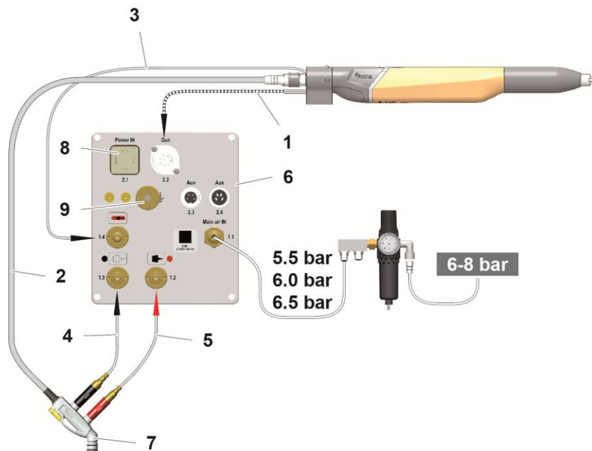
Fig. 7: Connection instructions – overview
