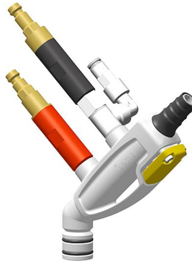
fig. 1: Powder injector with coded quick release connections
