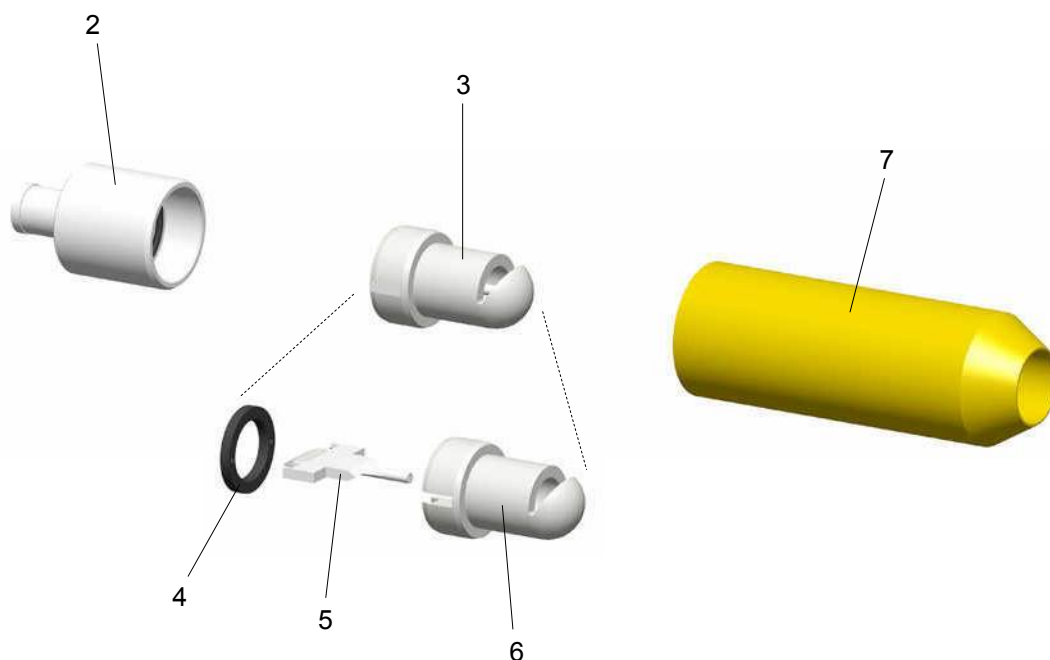
OptiGun GA03-E – Flat jet nozzle NF29-E-60°
