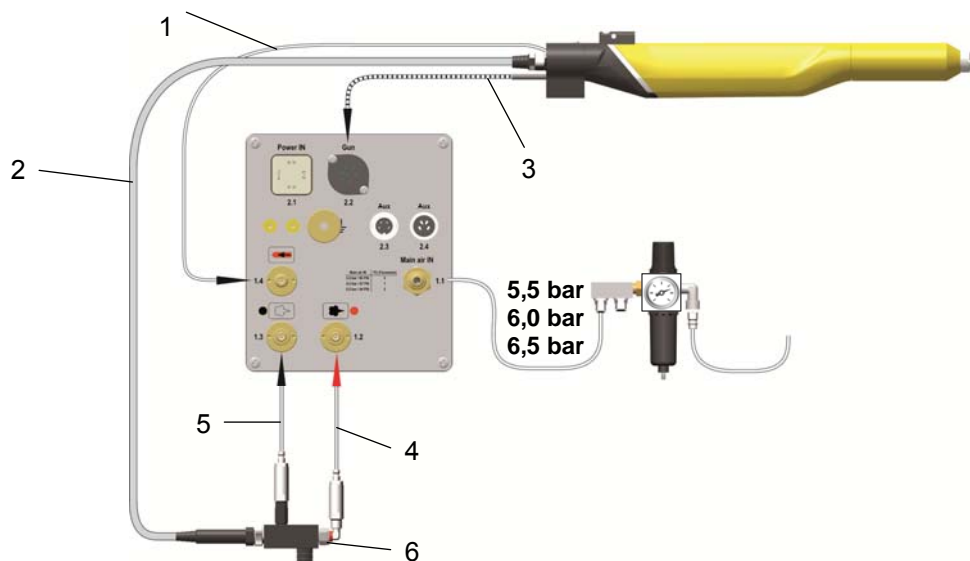
OptiGun GA03-E Enamel automatic gun - Connection instructions – overview
