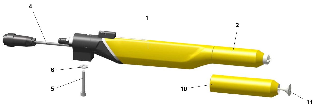
OptiGun GA03-E – complete
