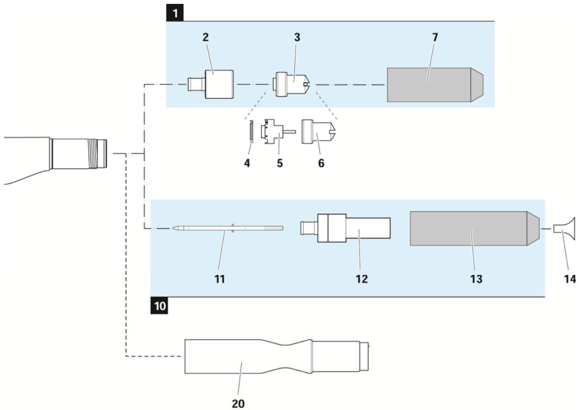
OptiGun GA03-E – Nozzle combinations
